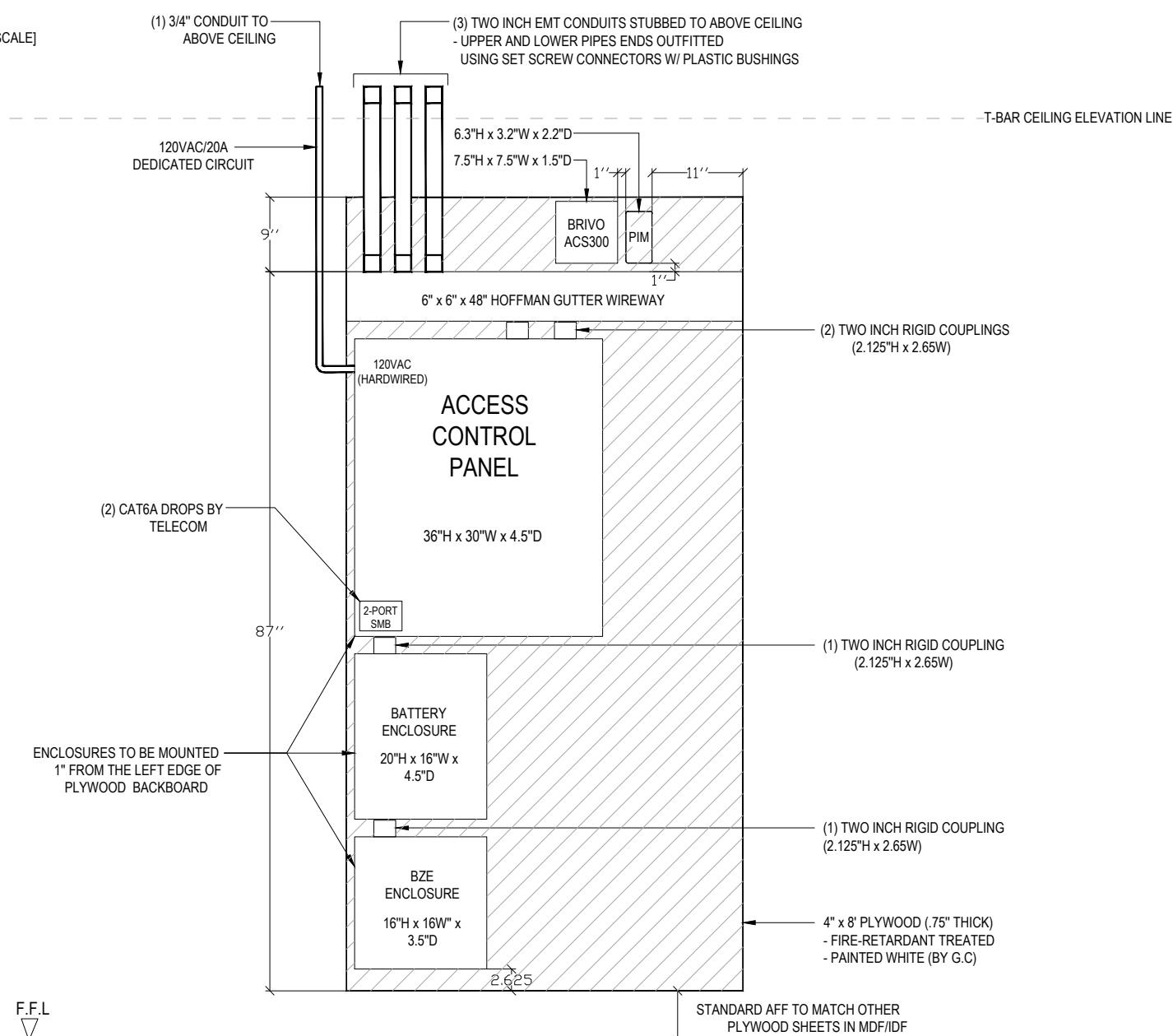
0.1 MDF LOWER LEVEL SOUTH
