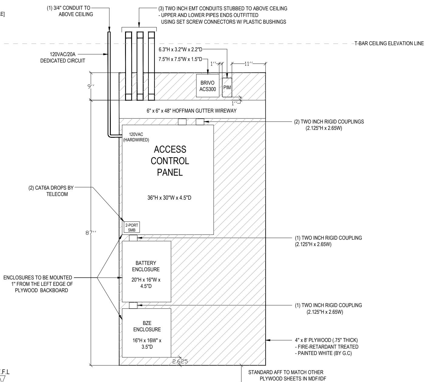
0.2 IDF LOWER LEVEL NORTH
