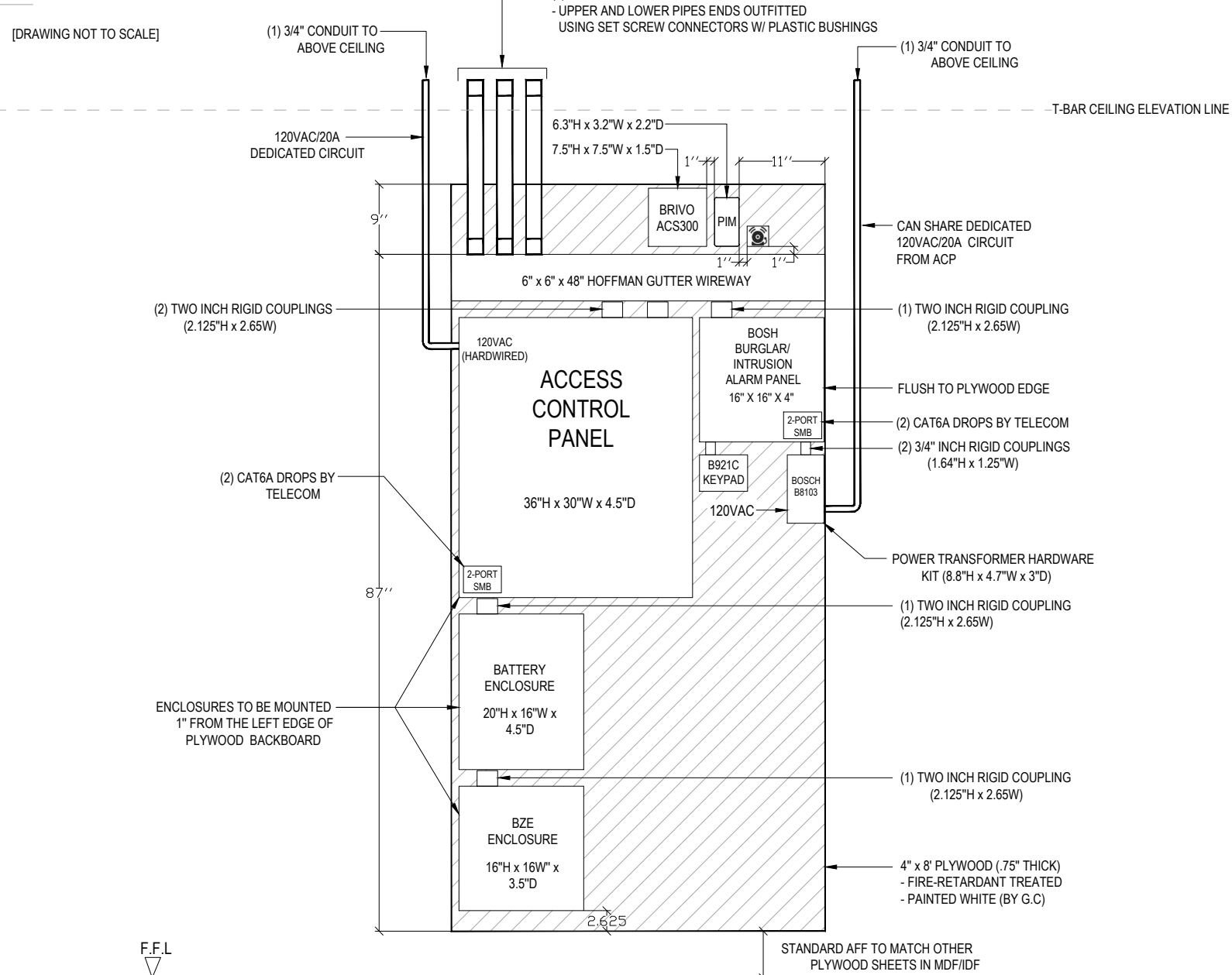
1.2 IDF LEVEL 1 NORTH
