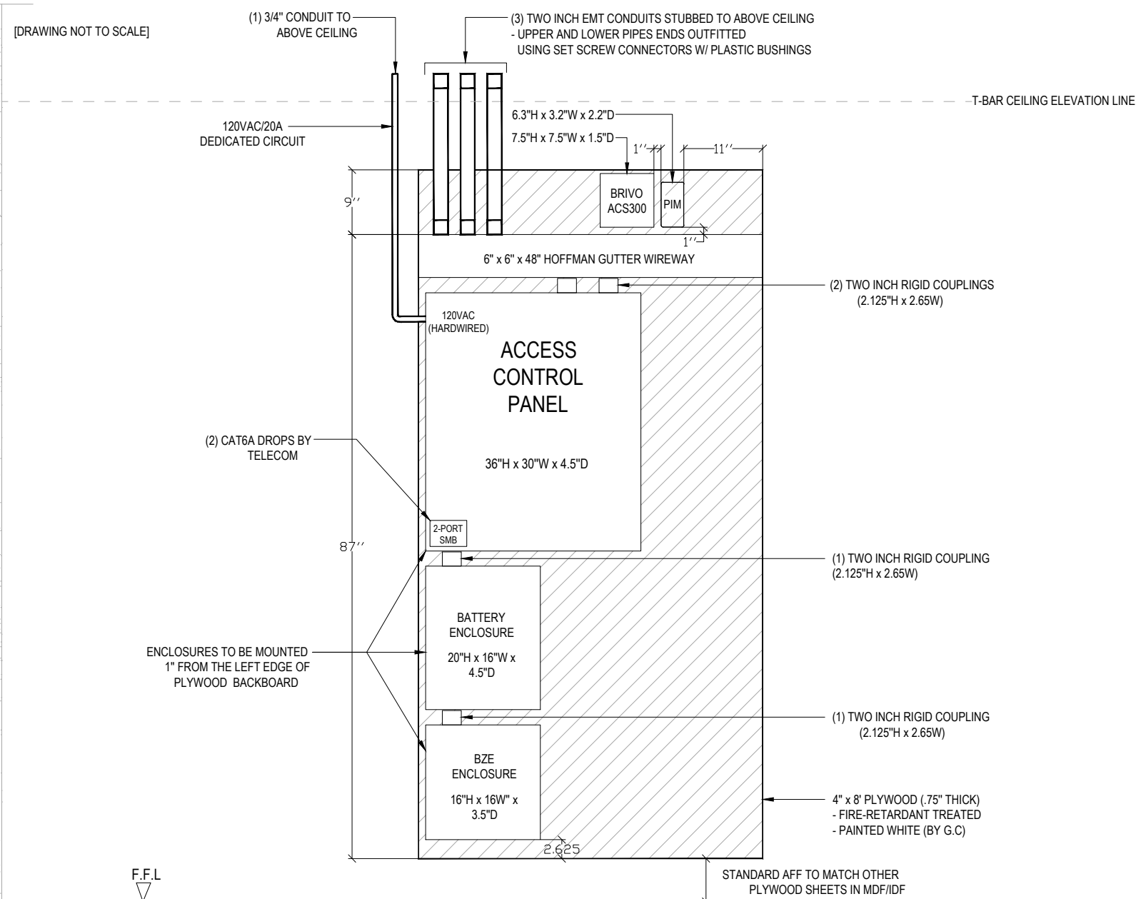
1.1 IDF LEVEL 1 SOUTH
